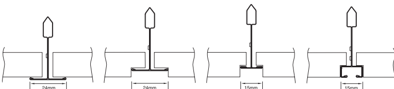
Square Lay-in with Peakform Grid
