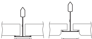
Square Lay-in with PeakForm Grid
