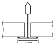
Square Lay-in with Peakform Grid
