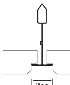
Beveled Tegular with PeakForm Suprafine XL Grid
