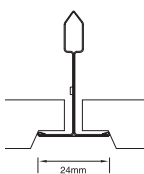
Angled Tegular with PeakForm Prelude XL Grid
